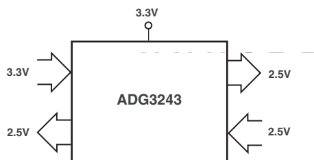
Figure 5. 3.3 V to 2.5 V Voltage Translation
