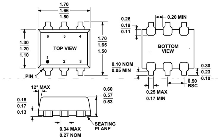
Figure 37. 6-Lead Small Outline Transistor Package [SOT-66] (RY-6-1)
