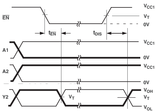
Figure 3. Y2 Enable and Disable Times
