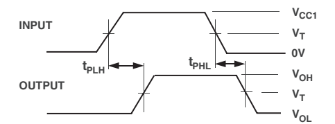
Figure 1. Propagation Delay
