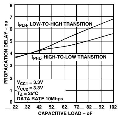
TPC 14. Propagation Delay vs. Capacitive Load, A1-Y
