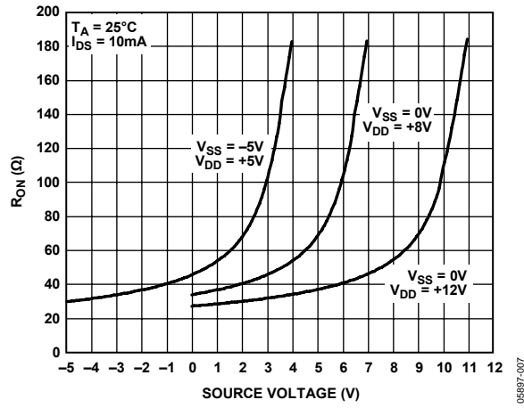
Figure 4. Signal Range
