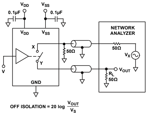
Figure 30. Off Isolation
