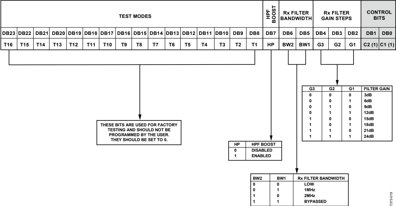
Figure 26. Rx Latch
