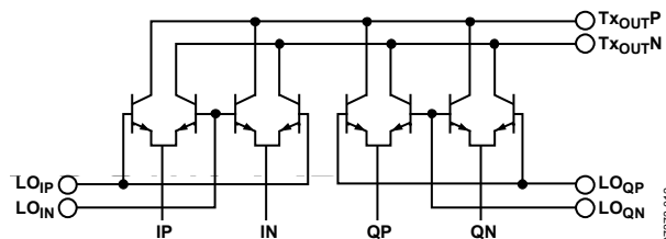
Figure 20. Tx Section
