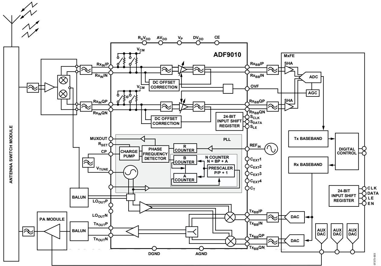
Figure 27. Applications Diagram
