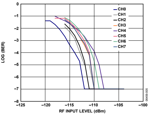
Figure 5. Sensitivity Plot
