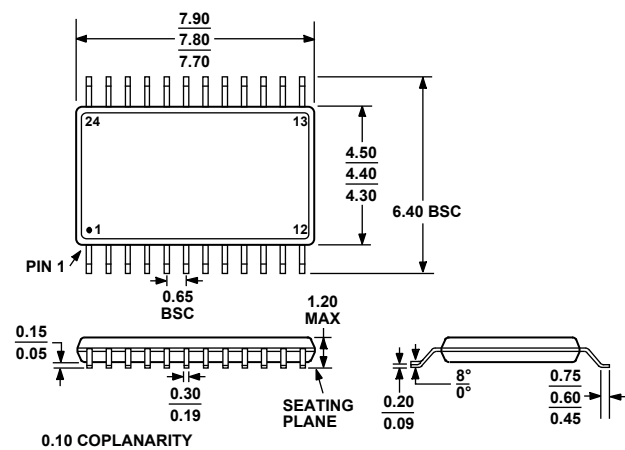
COMPLIANT TO JEDEC STANDARDS MO-153-AD Figure 8. 24-Lead Thin Shrink Small Outline Package [TSSOP] (RU-24) Dimensions shown in millimeters
