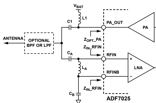
Figure 32. ADF7025 with Internal Rx/Tx Switch
