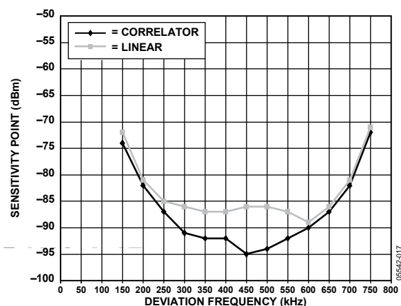
Figure 16. Sensitivity vs. Mod Index (Data Rate = 384 kbps, Baseband Filter Bandwidth = \pm 600 kHz), for Both Demodulator Types
