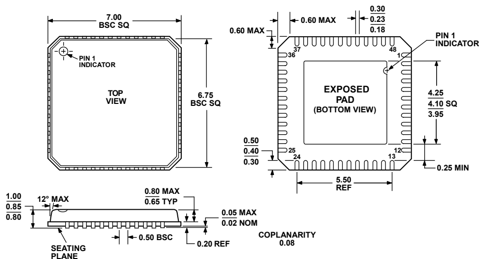
Figure 59. 48-Lead Lead Frame Chip Scale Package [LFCSP_VQ]
