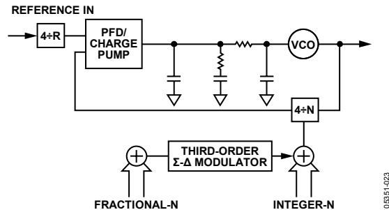
Figure 23. Fractional-N PLL
