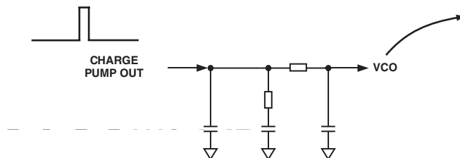
Figure 6. Typical Loop Filter Configuration—Third Order Integrator
