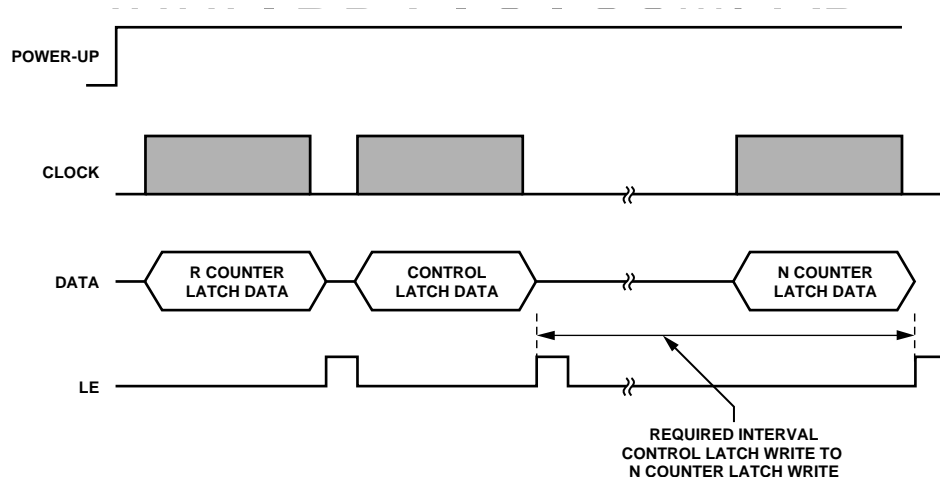
Figure 16. ADF4360-6 Power-Up Timing
