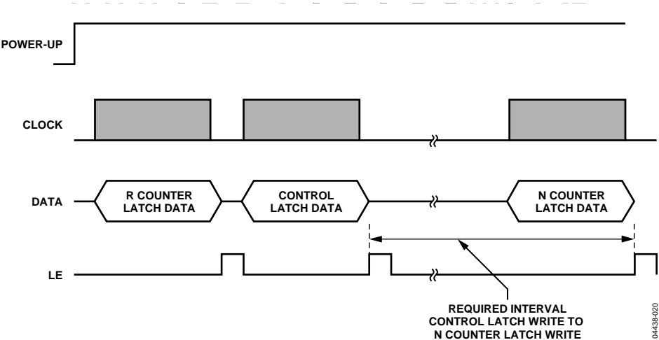
Figure 16. ADF4360-4 Power-Up Timing
