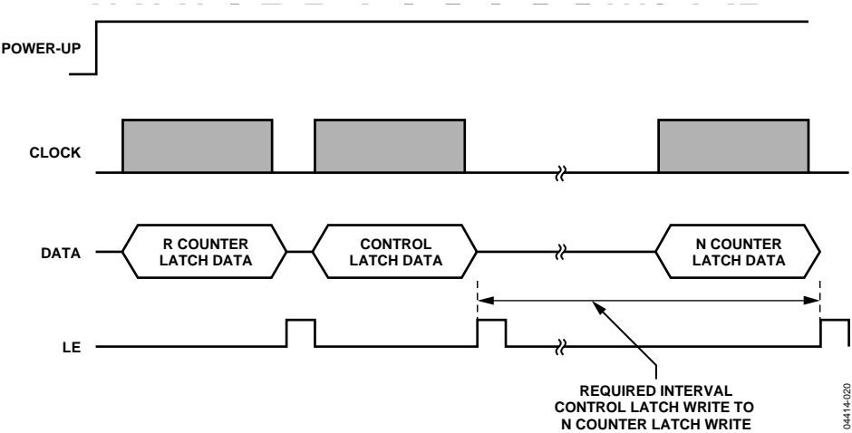
Figure 16. ADF4360-1 Power-Up Timing
