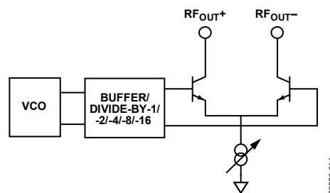
Figure 15. Output Stage
