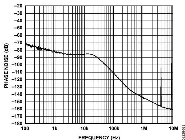
Figure 6. Fractional-N Phase Noise and Spur Performance; Low Spur Mode; GSM1800 Band, VCOOUT = 1850 MHz, REF_{IN} = 104 MHz, PFD = 13 MHz, Loop Filter Bandwidth = 15 kHz, Channel Spacing = 200 kHz (Note That Fractional Spurs Are Removed and Only the Integer Boundary Spurs Remain in Low Spur Mode)
