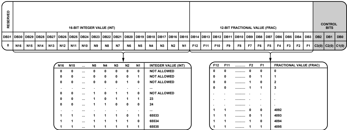
Figure 17. Register 0 (R0)
