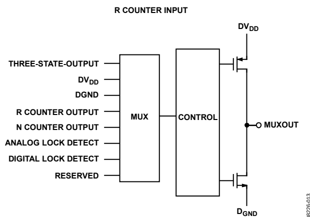
Figure 14. MUXOUT Schematic
