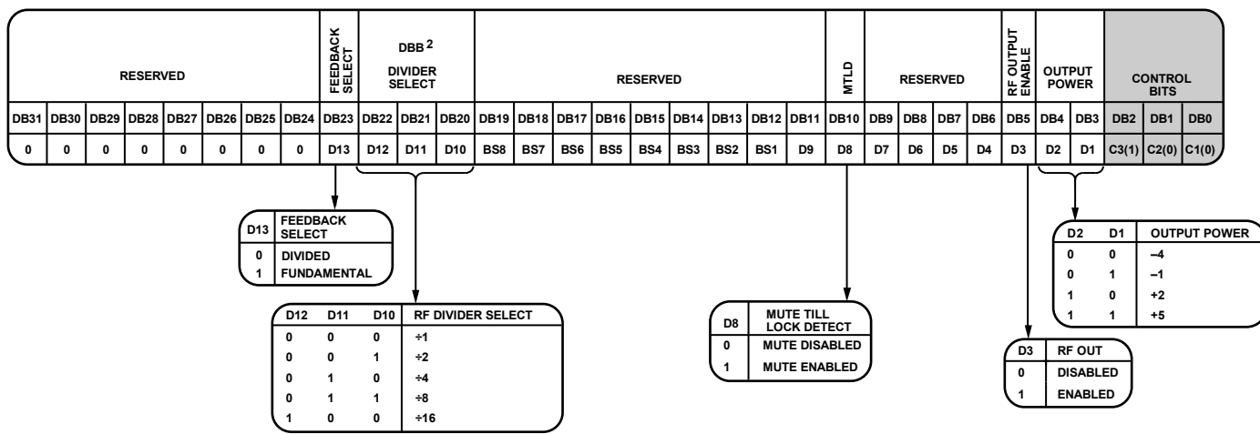
Figure 21. Register 4 (R4)
