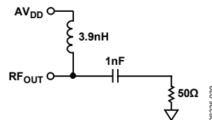
Figure 31. Optimum ADF4150 Output Stage
