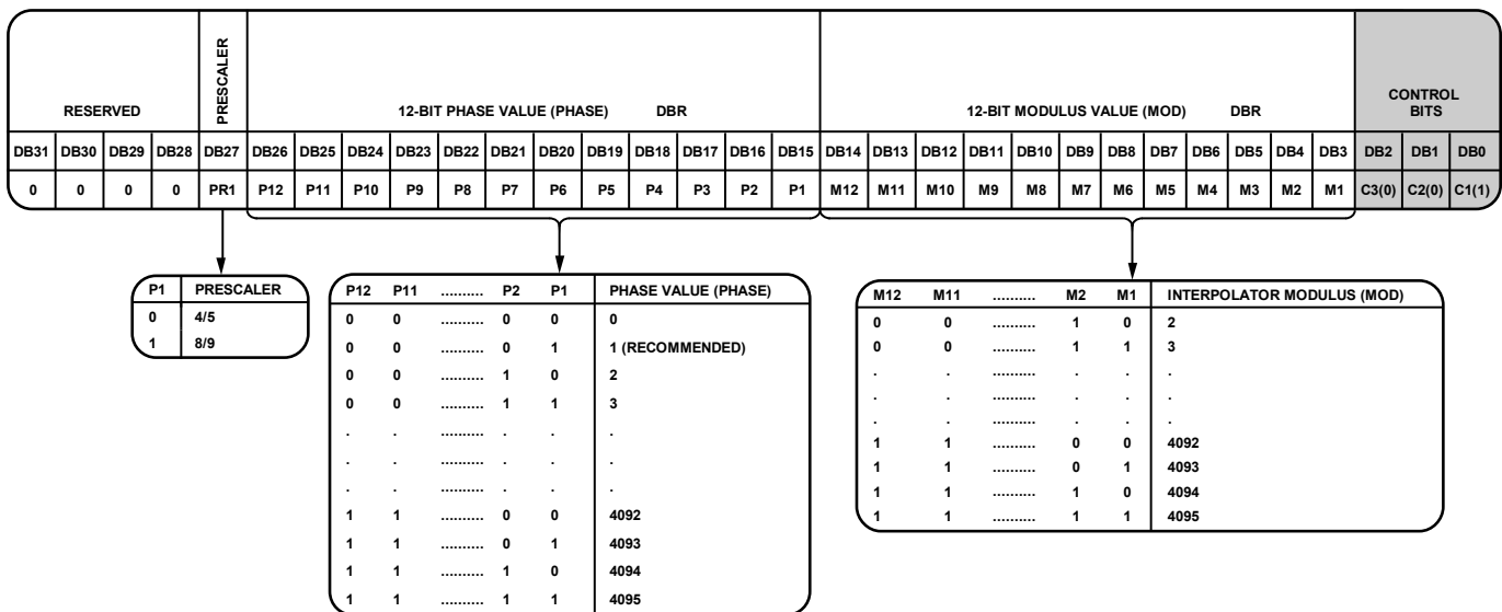
Figure 18. Register 1 (R1)
