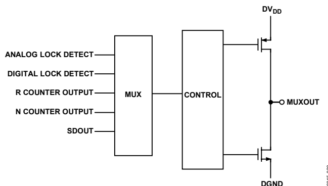
Figure 14. MUXOUT Circuit
