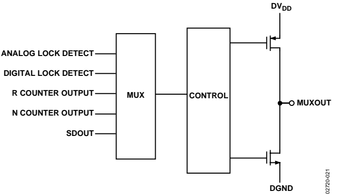
Figure 21. MUXOUT Circuit
