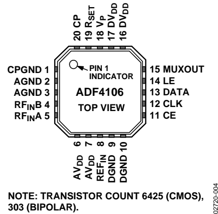
Figure 4. 20-Lead LFCSP_VQ Pin Configuration
