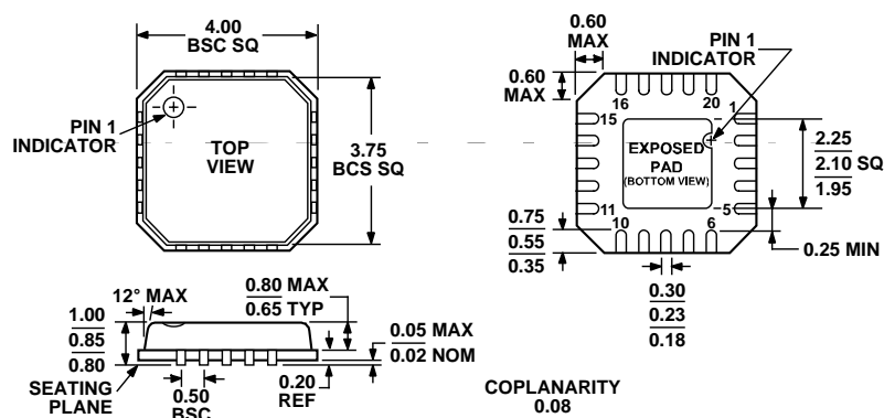
Figure 26. 20-Lead Lead Frame Chip Scale Package [LFCSP_VQ] 4 mm × 4 mm Body, Very Thin Quad (CP-20-1) Dimensions shown in millimeters
