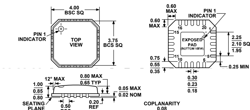
Figure 25. 20-Lead Lead Frame Chip Scale Package [LFCSP_VQ] (CP-20-1)
