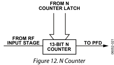
Figure 12. N Counter
