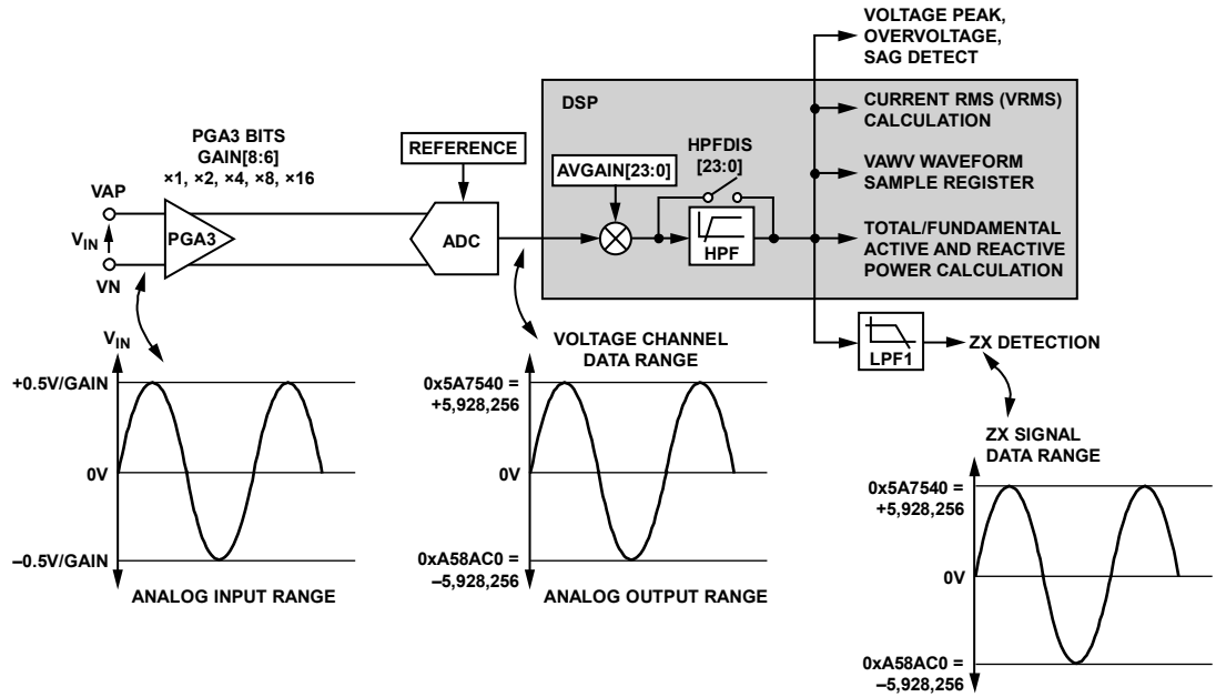
Figure 38. Voltage Channel Datapath
