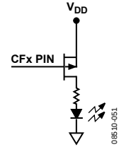
Figure 71. CFx Pin Recommended Connection
