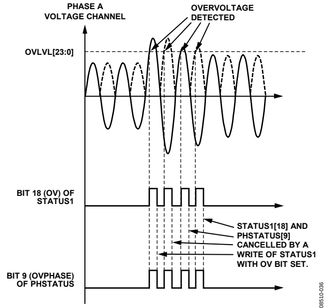
Figure 50. Overvoltage Detection
