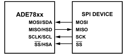
Figure 83. Connecting ADE78xx SPI with an SPI Device
