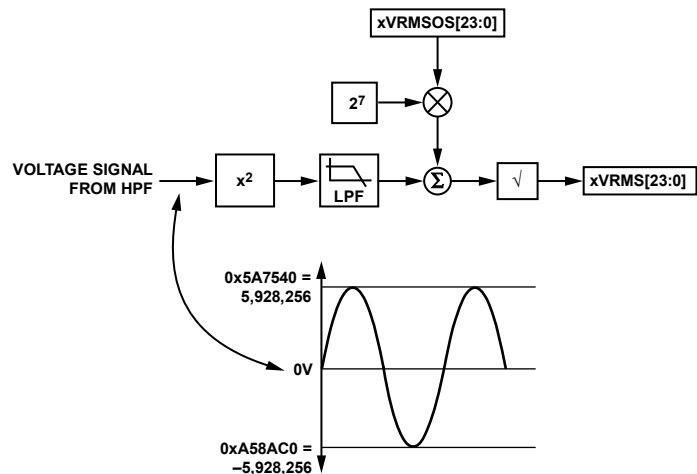
Figure 58. Voltage RMS Signal Processing
