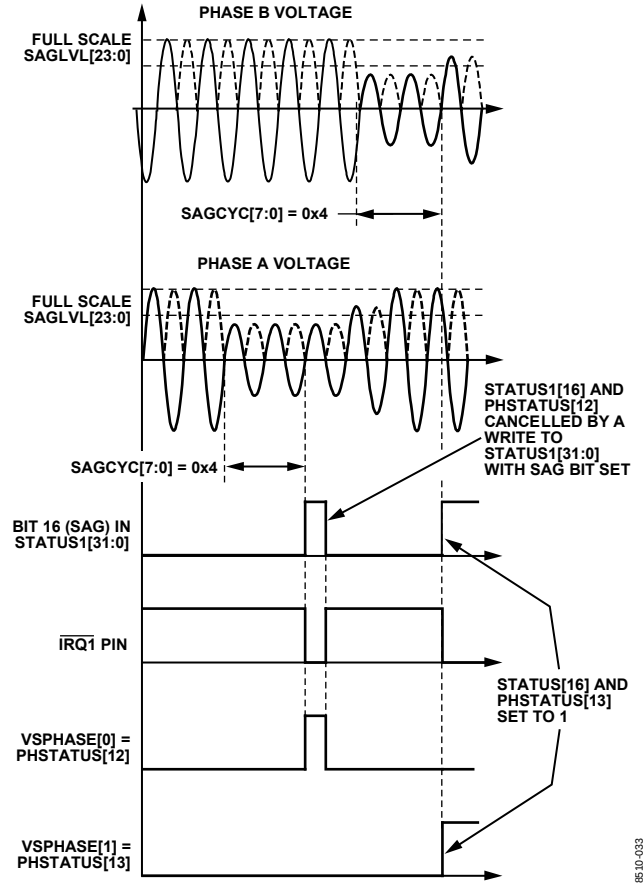
Figure 47. SAG Detection
