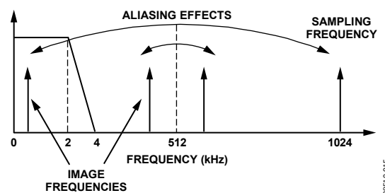
Figure 30. Aliasing Effects
