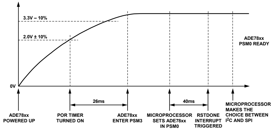
Figure 24. Power-Up Procedure
