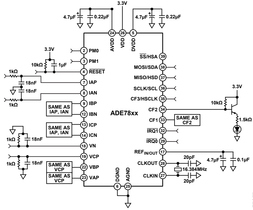
Figure 22. Test Circuit
