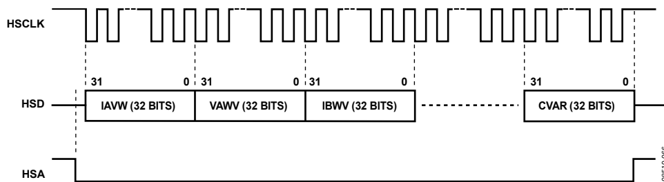
Figure 87. HSDC Communication for HGAP = 0, HXFER[1:0] = 00, and HSAPO = 0; HSIZE is Irrelevant
