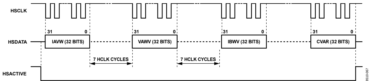
Figure 88. HSDC Communication for HSIZE = 0, HGAP = 1, HXFER[1:0] = 00, and HSAPO = 0
