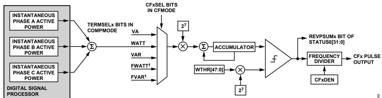
Figure 70. Energy-to-Frequency Conversion
