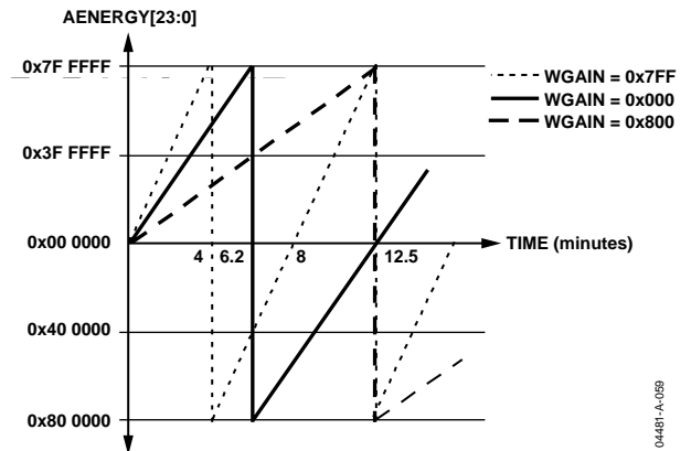
Figure 58. Energy Register Rollover Time for Full-Scale Power (Minimum and Maximum Power Gain)
