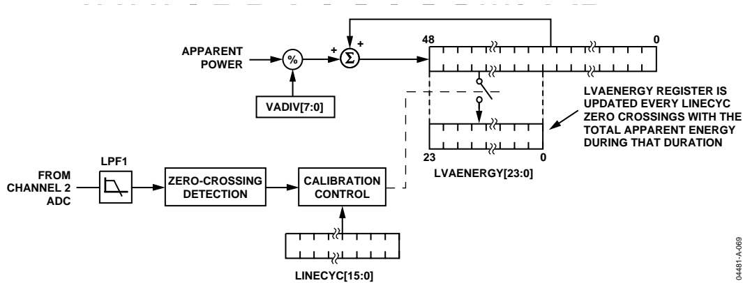
Figure 68. Apparent Energy Calibration
