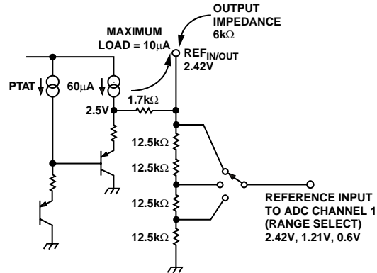
Figure 42. Reference Circuit Output
