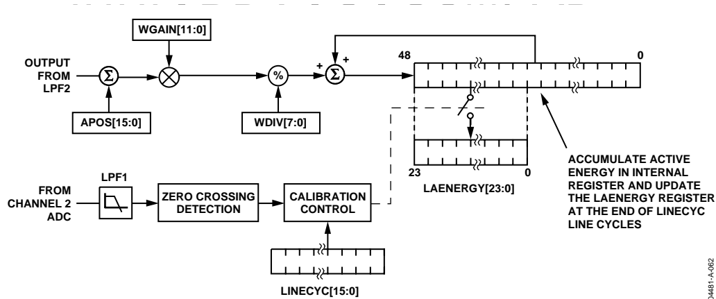
Figure 61. Energy Calculation Line Cycle Energy Accumulation Mode
