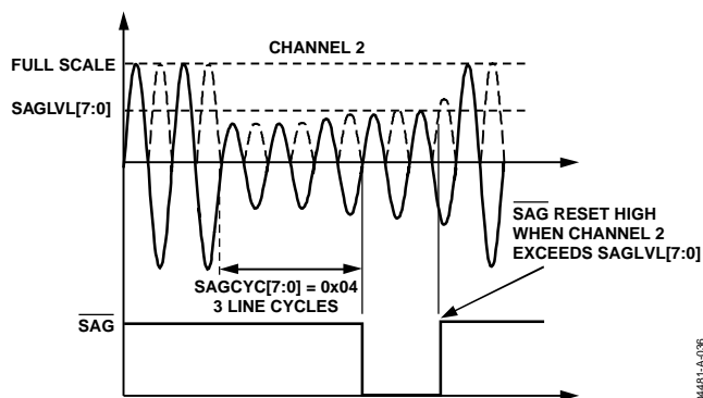
Figure 35. Sag Detection
