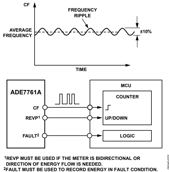
Figure 35. Interfacing the ADE7761A to an MCU
