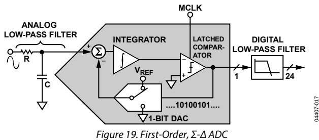
Figure 19. First-Order, \Sigma - \Delta ADC
