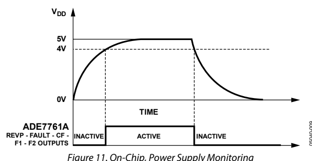
Figure 11. On-Chip, Power Supply Monitoring
