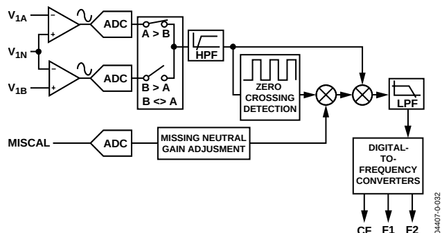
The ADE7761 detects a missing neutral condition by continuously monitoring the voltage channel input ( V_{2P}-V_{2N} ). The FAULT pin is held high when a missing neutral condition is detected. In this mode, the ADE7761 continues to bill the energy based on the signal level on the current channel (see Figure 30). The billing rate or frequency outputs can be adjusted by changing the dc level on the MISCAL pin.
