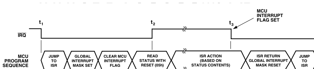
Figure 17. Interrupt Management
