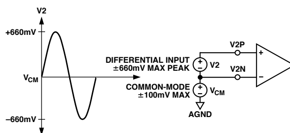
Figure 5. Maximum Signal Levels, Channel 2
