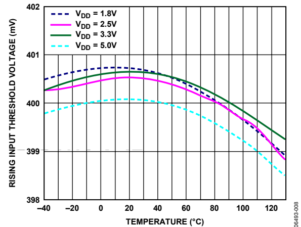
Figure 8. Rising Input Threshold Voltage vs. Temperature
