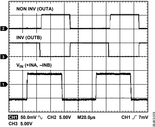
Figure 29. Noninverting and Inverting Comparators Propagation Delay
