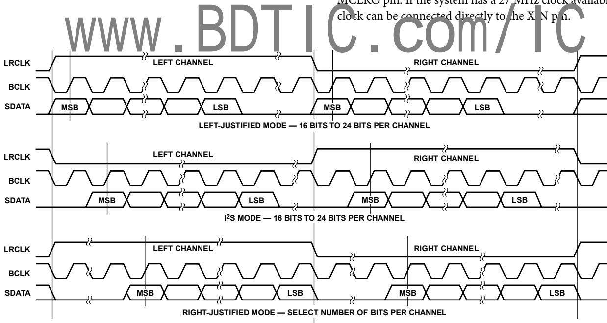
Figure 51. Serial Data Modes
