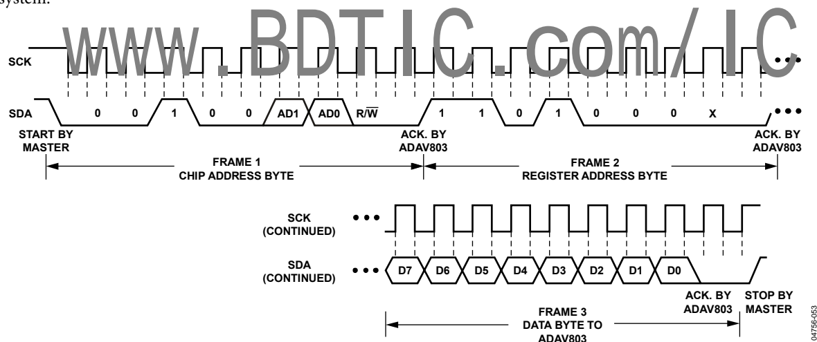
Figure 53. Writing to the DAC Left Volume Register in I 2 C
