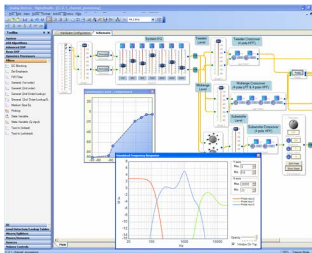
Figure 29. SigmaStudio Screen Shot
