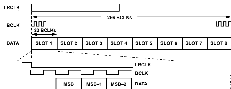
Figure 34. TDM Mode
