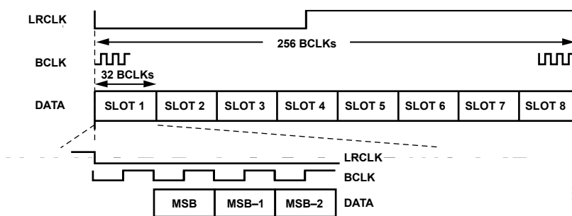
Figure 34. TDM Mode
