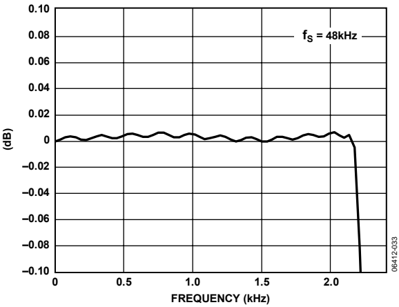
Figure 10. DAC Pass-Band Filter Response, f_s = 48\text{ kHz}
