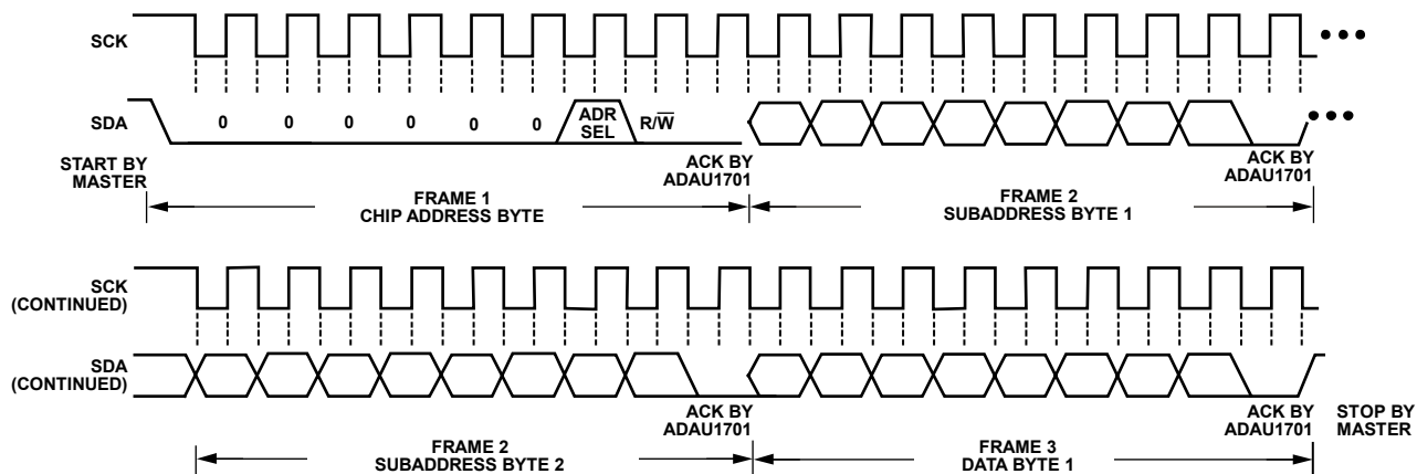
Figure 20. I 2 C Write to ADAU1701 Clocking
