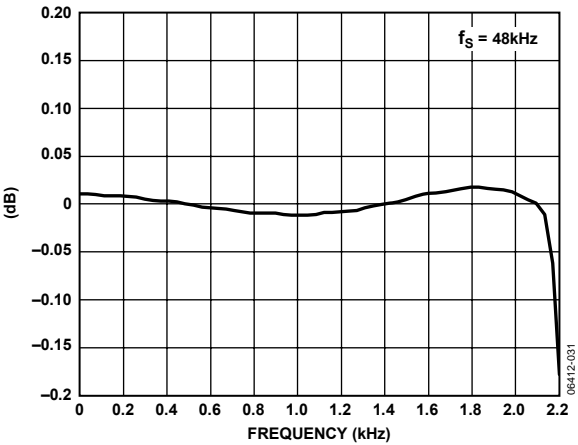
Figure 8. ADC Pass-Band Filter Response, f_s = 48\text{ kHz}
