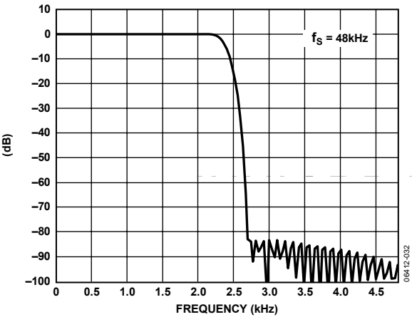
Figure 9. ADC Stop-Band Filter Response, f_s = 48\text{ kHz}
