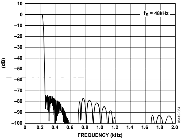
Figure 11. DAC Stop-Band Filter Response, f_s = 48\text{ kHz}
