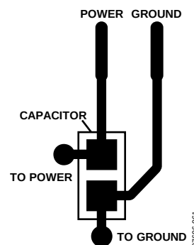
Figure 62. Recommended Power Supply Bypass Capacitor Layout
