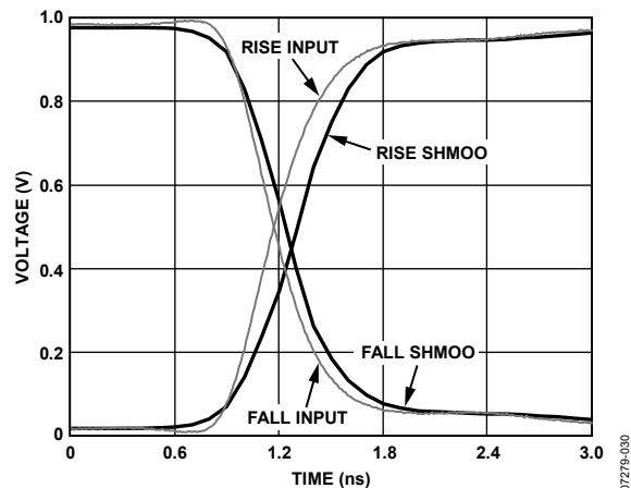
Figure 30. Comparator Shmoo, 1.0 V Input, 0.7 ns (10% to 90%) Input, 50 \Omega Terminated
