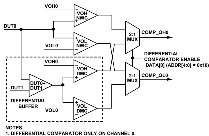
Figure 77. Comparator Block Diagram
