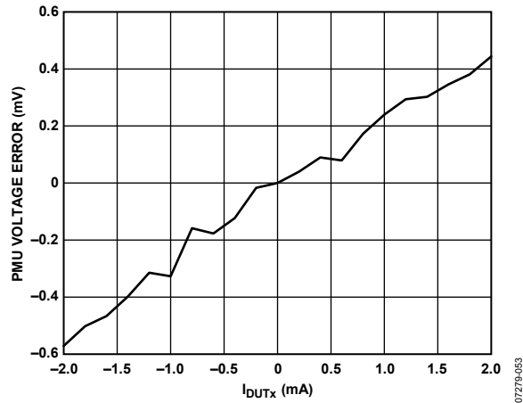
Figure 51. PMU FV Range B Output Voltage Error at -1.25 V vs. Output Current
