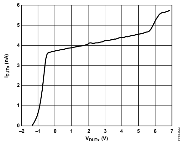
Figure 42. DUTx Pin Leakage in High-Z Mode
