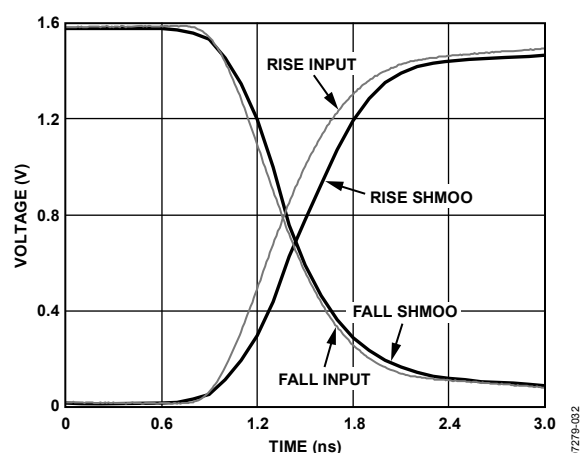
Figure 32. Comparator Shmoo, 1.5 V Input, 1.0 ns (10% to 90%) Input, 50 \Omega Terminated
