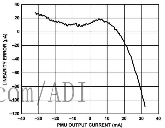
Figure 43. PMU Force Current Range A Linearity
