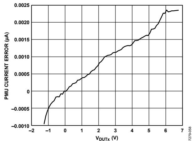
Figure 56. PMU FI Range E Output Current Error at -2 \mu A vs. Output Voltage; Output Voltage Is Pulled Externally
