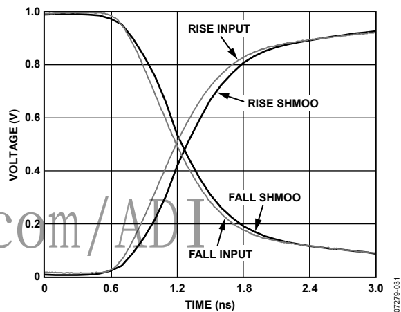
Figure 31. Comparator Shmoo, 1.5 V Input, 1.0 ns (10% to 90%) Input, 50 \Omega Terminated
