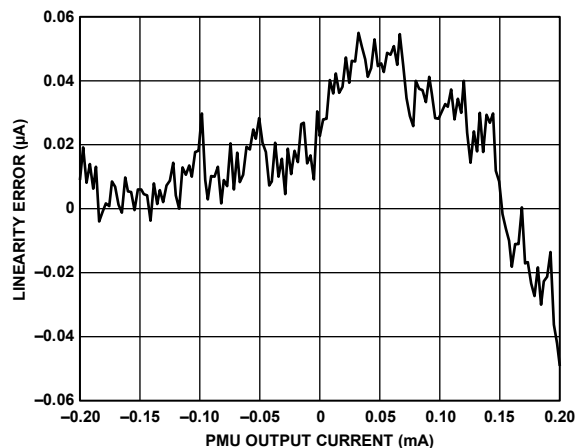
Figure 45. PMU Force Current Range C Linearity
