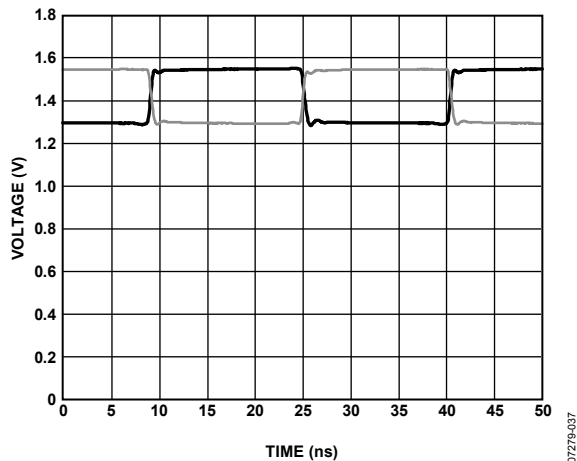
Figure 35. Comparator Output Waveform, COMP_QH0P, COMP_QH0N
