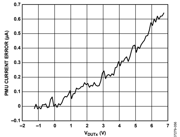
Figure 54. PMU FI Range B Output Current Error at -2 mA vs. Output Voltage; Output Voltage Is Pulled Externally
