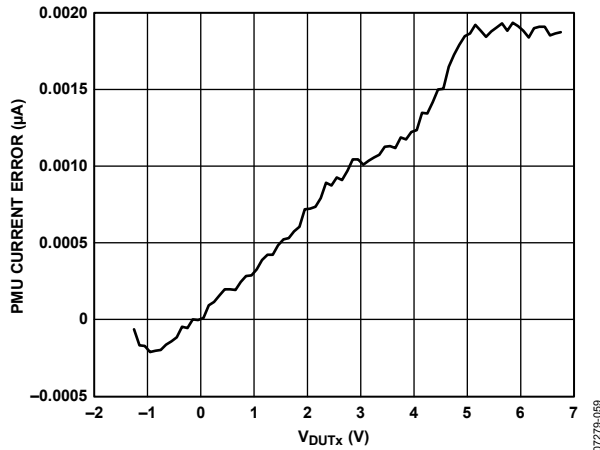
Figure 57. PMU FI Range E Output Current Error at +2 \mu A vs. Output Voltage; Output Voltage Is Pulled Externally
