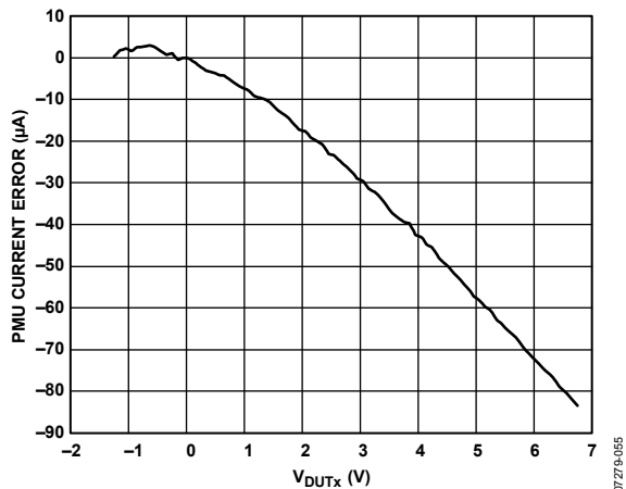
Figure 53. PMU FI Range A Output Current Error at +32 mA vs. Output Voltage; Output Voltage Is Pulled Externally
