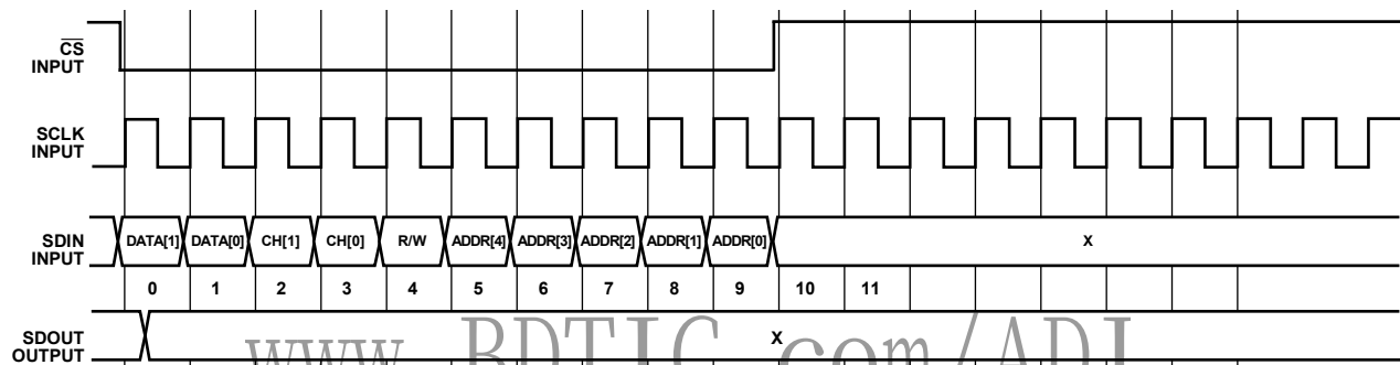
Figure 69. 16-Bit SPI Write
