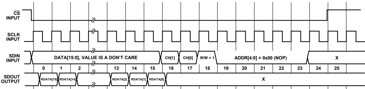
Figure 73. SPI Read—Details of Read Out
