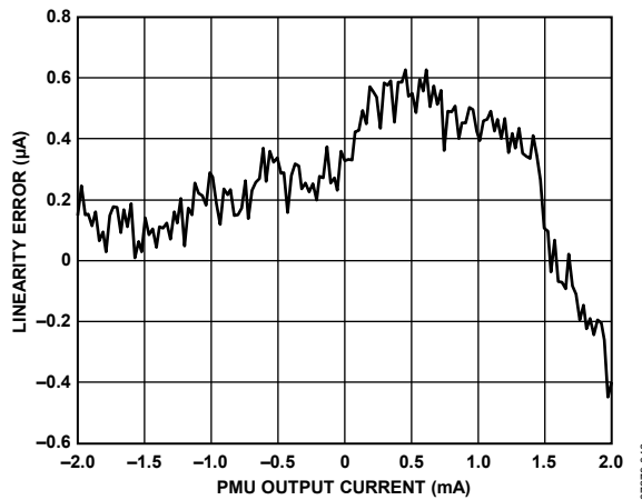
Figure 44. PMU Force Current Range B Linearity
