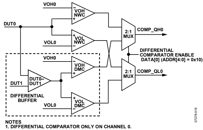
Figure 89. Comparator Block Diagram
