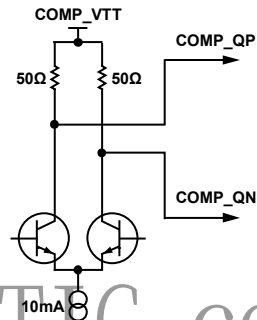
Figure 90. Comparator Output Scheme
