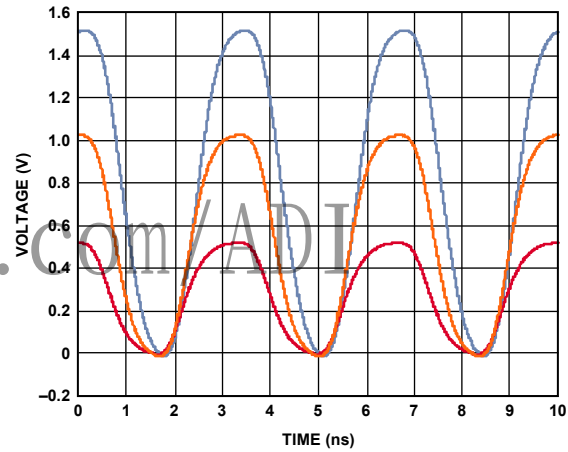
Figure 7. 300 MHz Driver Response; V_H = 1.0\text{ V}, 2.0\text{ V}, 3.0\text{ V} ; V_L = 0.0\text{ V} ; 50\ \Omega Termination
