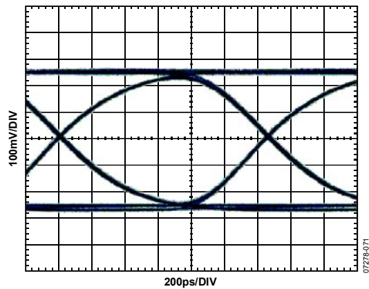
Figure 71. Eye Diagram, 800 Mbps, PRBS31; VH = 1.0 V; VL = 0.0 V
