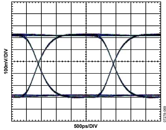
Figure 69. Eye Diagram, 400 Mbps, PRBS31; VH = 1.0 V; VL = 0.0 V
