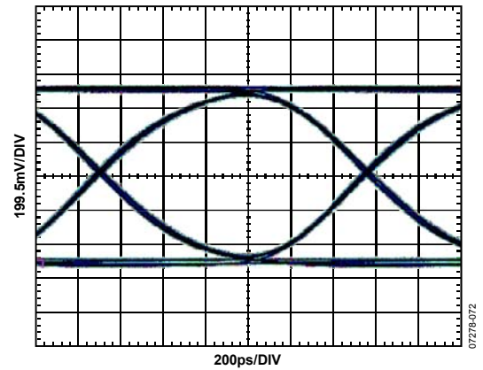
Figure 72. Eye Diagram, 800 Mbps, PRBS31; VH = 2.0 V; VL = 0.0 V
