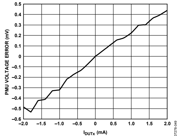
Figure 54. PMU Force Voltage Range B Output Voltage Error at -2.0 V vs. Output Current
