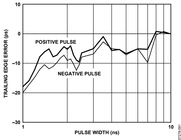
Figure 35. Comparator Minimum Pulse Width Input; 1.0 V Swing; 200 ps (10%/90%)
