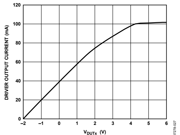
Figure 26. Driver Output Current Limit; Driver Programmed to -2.0 V; VOUTx Swept from -2.0 V to +6.0 V
