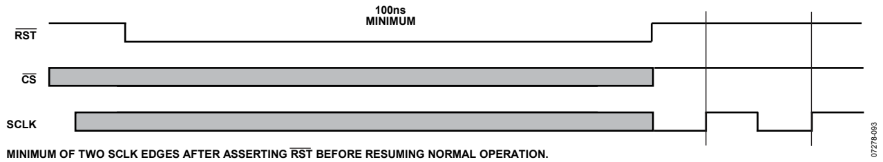
Figure 86. Reset Operation
