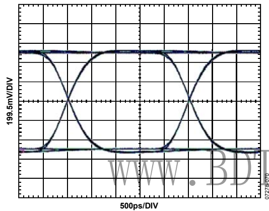
Figure 70. Eye Diagram, 400 Mbps, PRBS31; VH = 2.0 V; VL = 0.0 V
