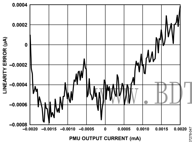
Figure 52. PMU Force Current Range E Linearity
