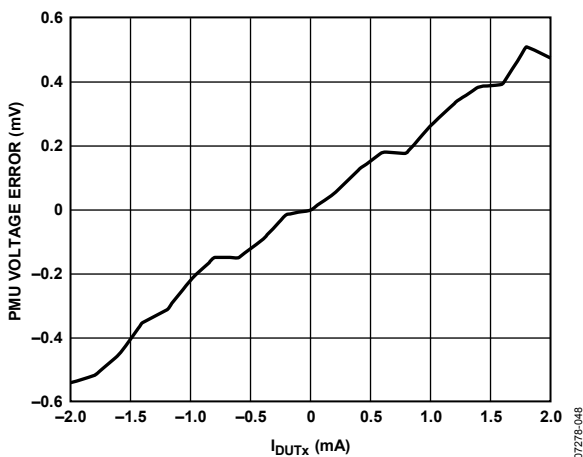
Figure 53. PMU Force Voltage Range B Output Voltage Error at 6.0 V vs. Output Current
