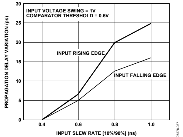
Figure 36. Comparator Slew Rate Dispersion
