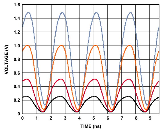
Figure 8. 400 MHz Driver Response; V_H = 0.5\text{ V}, 1.0\text{ V}, 2.0\text{ V}, 3.0\text{ V} ; V_L = 0.0\text{ V} ; 50\ \Omega Termination
