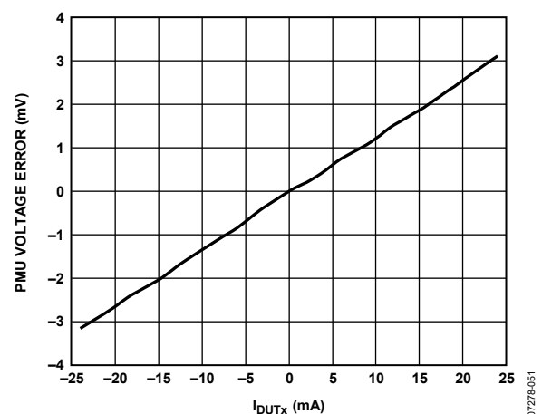
Figure 56. PMU Force Voltage Range A Output Voltage Error at -2.0 V vs. Output Current
