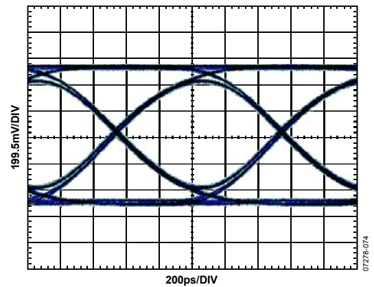
Figure 74. Eye Diagram, 1000 Mbps, PRBS31; VH = 2.0 V; VL = 0.0 V
