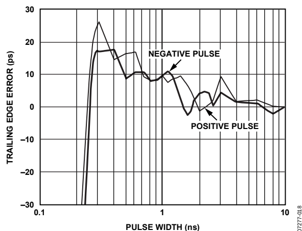
Figure 18. 3 V Minimum Pulse Width ( V_{Hx} = 3.0\text{ V} , V_{Lx} = 0.0\text{ V} ), CLC Disabled
