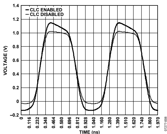
Figure 8. V_{Hx} = 2.0\text{ V} , V_{Lx} = 0.0\text{ V} , 1.0\text{ GHz} Waveform, CLC Disabled and Enabled
