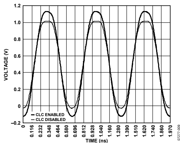
Figure 6. V_{Hx} = 2.0\text{ V} , V_{Lx} = 0.0\text{ V} , 1.5\text{ GHz} Waveform, CLC Disabled and Enabled
