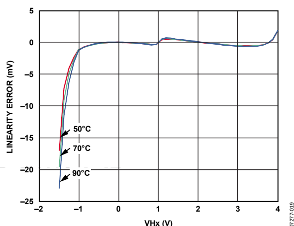
Figure 19. Driver Linearity ( V_{Hx} ), V_{Lx} = -1.1\text{ V} , V_{Tx} = 1.0\text{ V}
