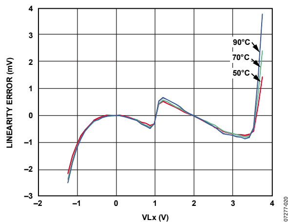
Figure 20. Driver Linearity ( V_{Lx} ), V_{Hx} = 3.6\text{ V} , V_{Tx} = 1.0\text{ V}
