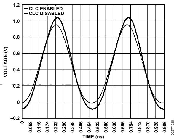
Figure 7. V_{Hx} = 2.0\text{ V} , V_{Lx} = 0.0\text{ V} , 2.0\text{ GHz} Waveform, CLC Disabled And Enabled
