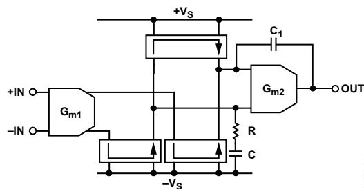
Figure 32. High Level Design Schematic
