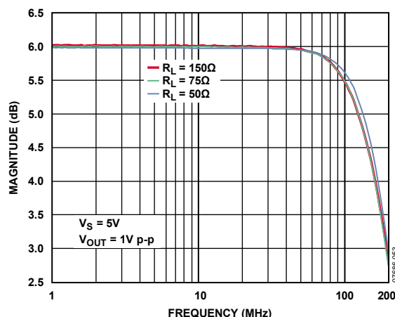
Figure 45. Large Signal Frequency Response for Various Loads
