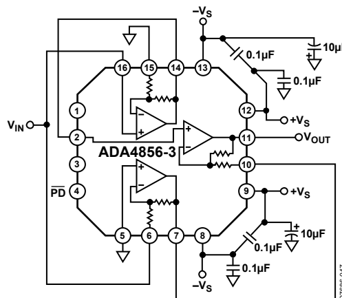
Figure 39. Gain of +5
