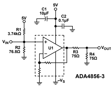
Figure 47. DC-Coupled Single Supply Video Driver Schematic
