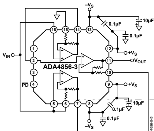
Figure 37. Gain of +3
