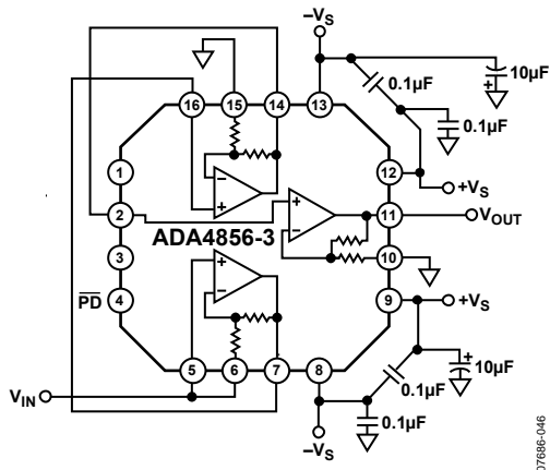
Figure 38. Gain of +4
