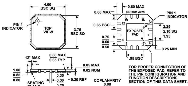
Figure 48.16-Lead Lead Frame Chip Scale Package [LFCSP_VQ] 4 mm × 4 mm Body, Very Thin Quad (CP-16-4)
