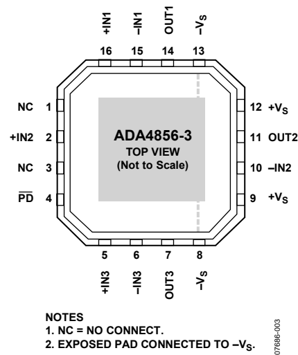
Figure 4. Pin Configuration
