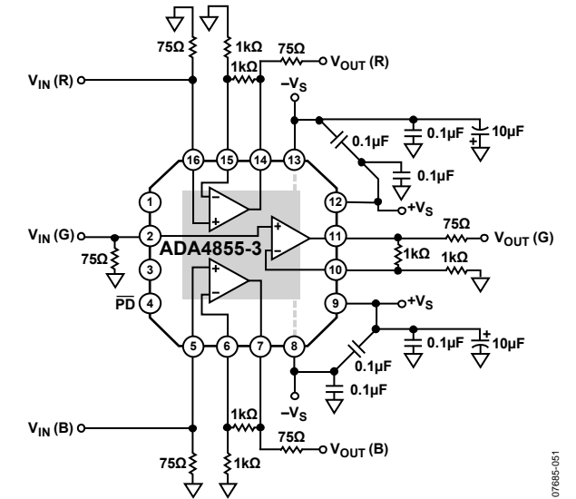
Figure 51. RGB Video Driver
