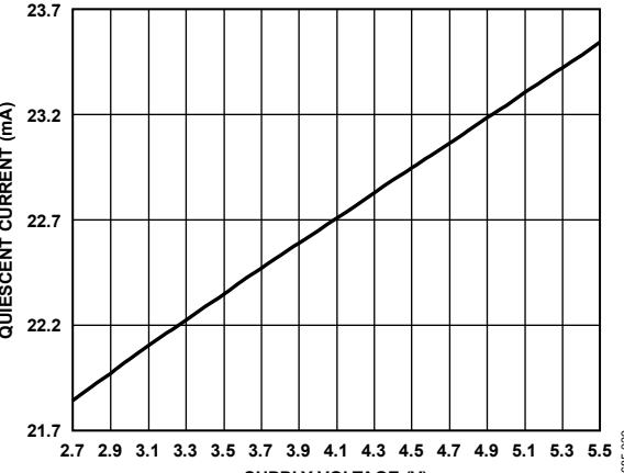
Figure 28. Quiescent Current vs. Supply Voltage
