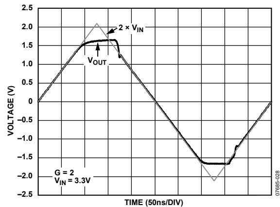
Figure 32. Output Overdrive Recovery
