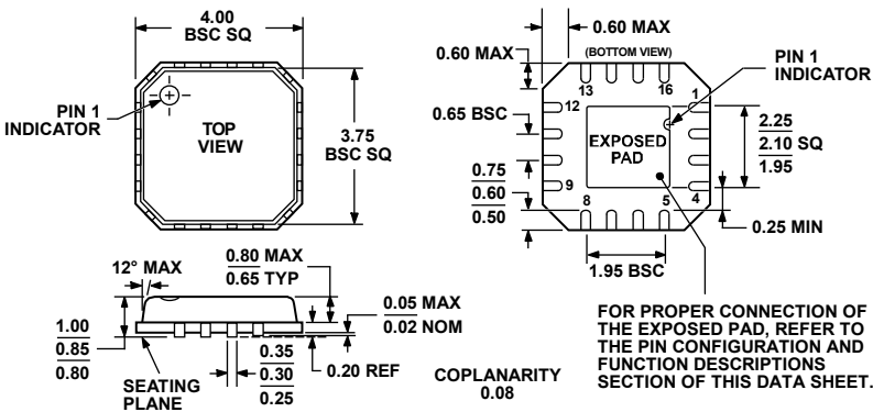
COMPLIANT TO JEDEC STANDARDS MO-220-VGGC Figure 56.16-Lead Lead Frame Chip Scale Package [LFCSP_VQ] 4 mm × 4 mm Body, Very Thin Quad (CP-16-4) Dimensions shown in millimeters
