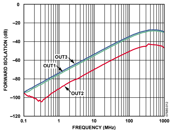
Figure 17. Forward Isolation vs. Frequency
