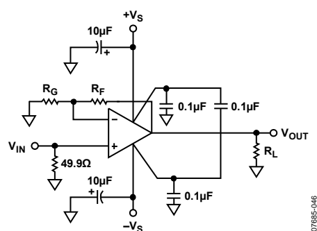
Figure 45. Typical Noninverting Gain Configuration
