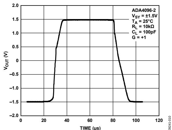
Figure 11. Large Signal Transient Response
