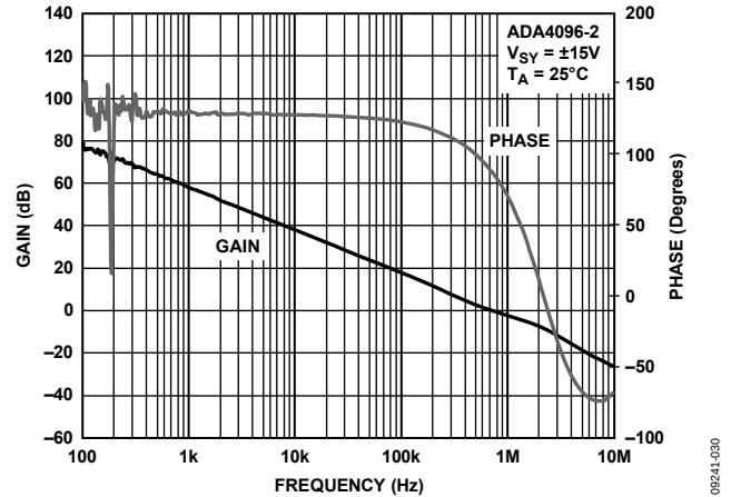
Figure 31. Open-Loop Gain and Phase vs. Frequency
