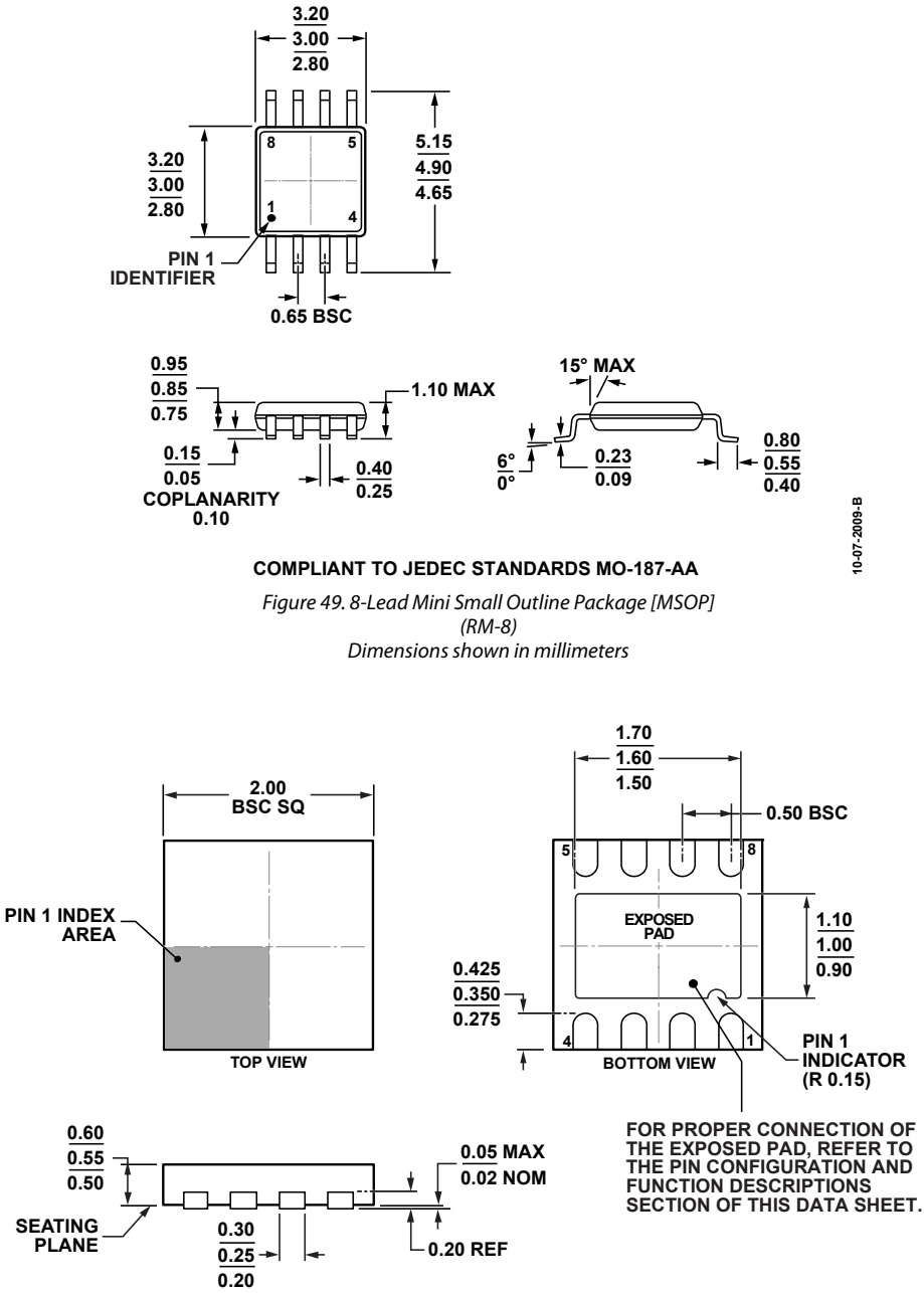
Figure 50. 8-Lead Lead Frame Chip Scale Package [LFCSP_UD] 2 mm × 2 mm Body, Ultra Thin, Dual Lead (CP-8-10) Dimensions shown in millimeters
