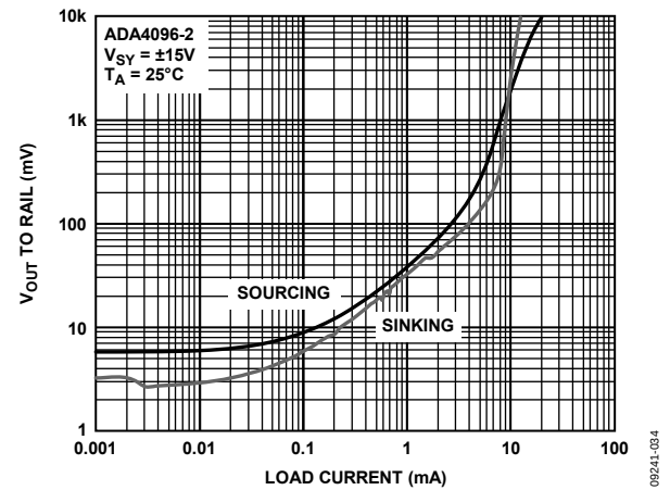
Figure 30. Dropout Voltage vs. Load Current
