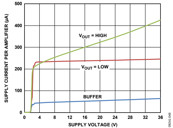
Figure 48. Comparator Supply Current
