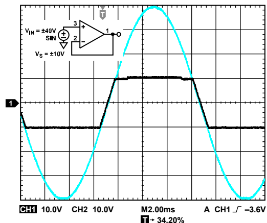
Figure 46. No Phase Reversal
