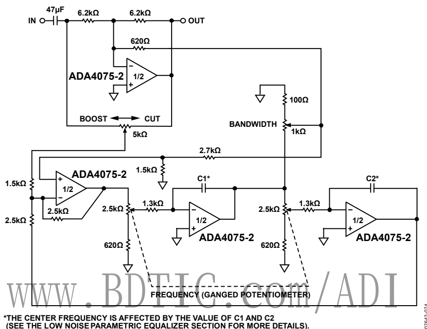
Figure 64. Low Noise Parametric Equalizer
