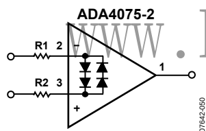
Figure 58. Input Protection
