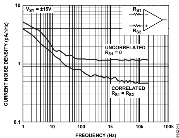
Figure 40. Current Noise Density
