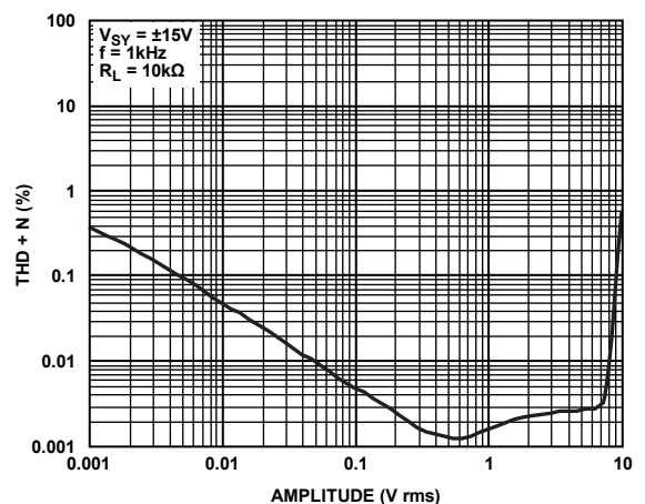
Figure 47. THD + N vs. Amplitude
