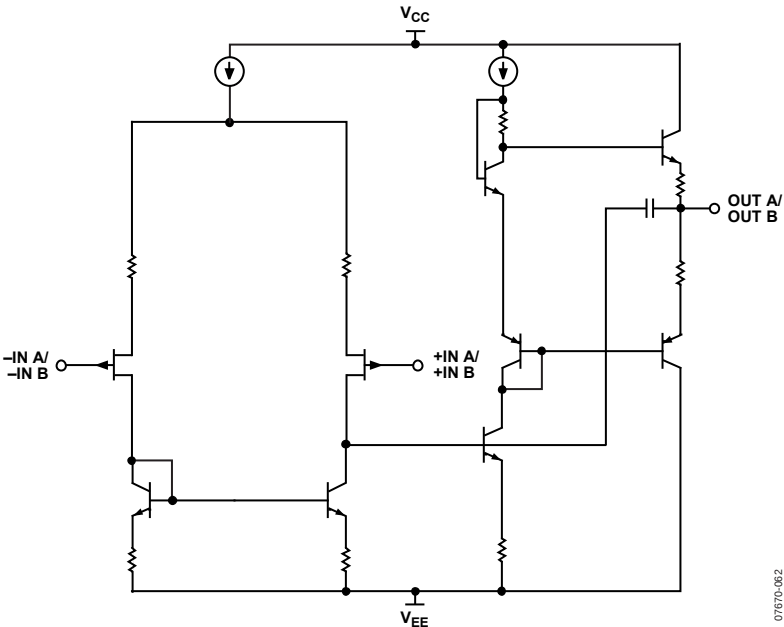
Figure 59. Simplified Schematic
