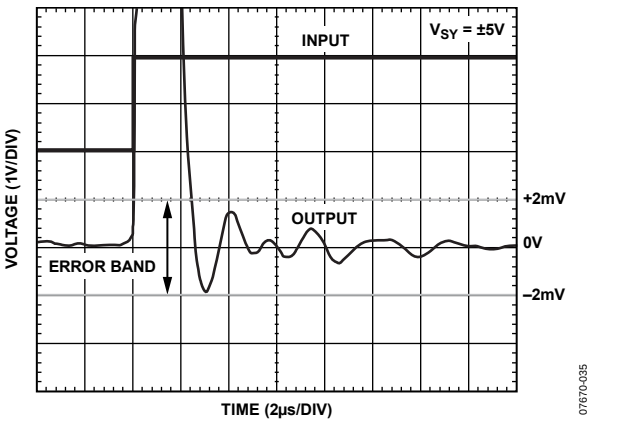
Figure 38. Positive Settling Time to 0.01%
