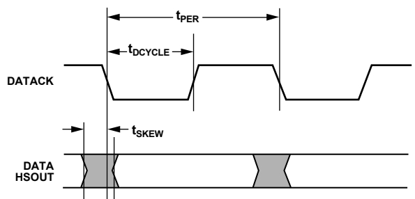
Figure 14. Output Timing
