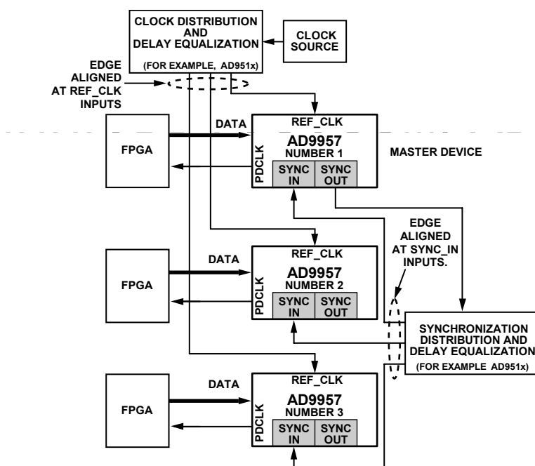
Figure 59. Multichip Synchronization Example
