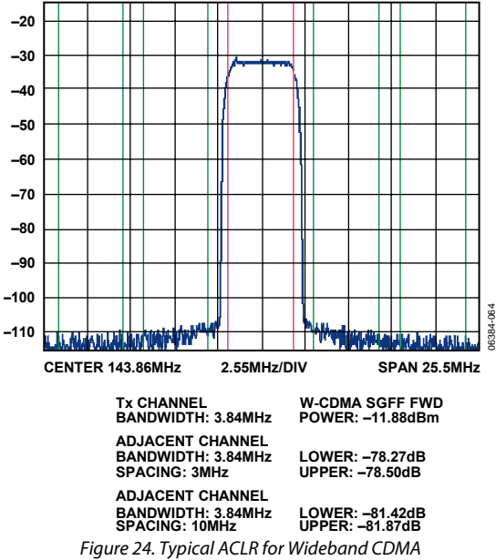
Figure 24. Typical ACLR for Wideband CDMA
