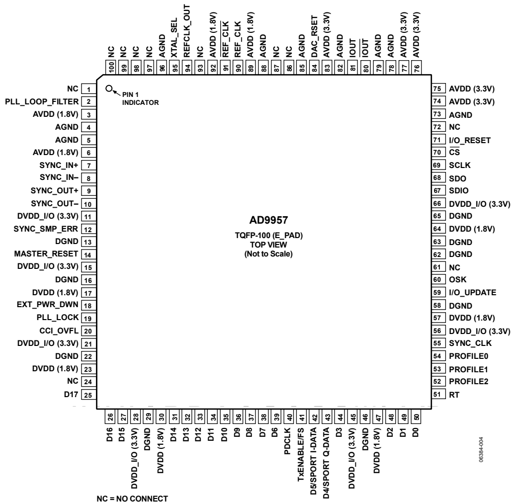
Figure 4. Pin Configuration
