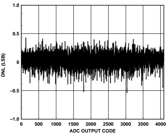
Figure 8. Typical DNL
