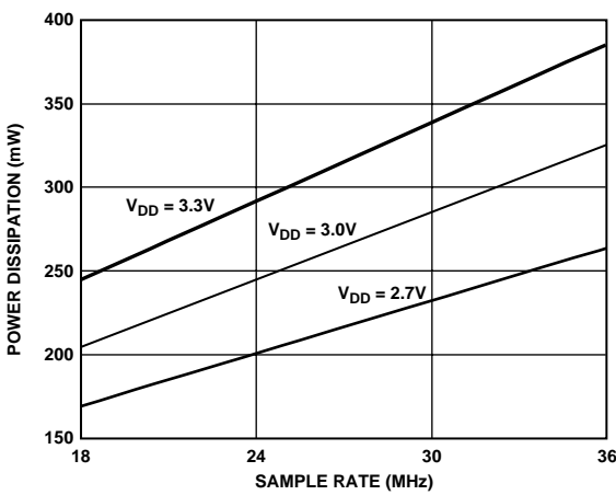
Figure 10. Power Curves
