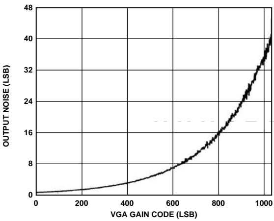
Figure 9. Output Noise vs. VGA Gain
