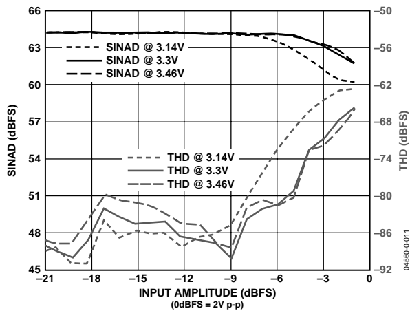
Figure 11. SINAD and THD vs. Input Amplitude and Supply ( f_{IN} = 8\text{ MHz} , LPF f_{-3\text{ dB}} = 26\text{ MHz} ; RxPGA = 0 dB)
