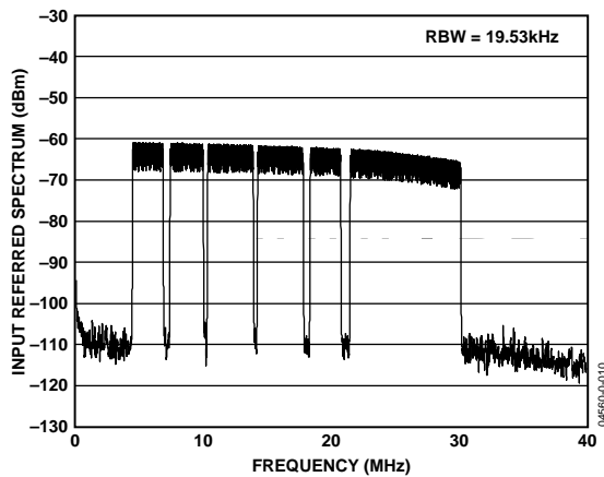
Figure 10. Spectral Plot with 4K FFT of 111-Carrier DMT Signal with PAR = 11\text{ dB} , P_{IN} = -33.7\text{ dBm} , LPF's f_{-3\text{ dB}} = 32\text{ MHz} and RxPGA = 36 dB
