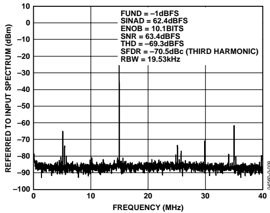
Figure 9. Spectral Plot with 4k FFT of Input Sinusoid with RxPGA = 0 dB and P_{IN} = 9\text{ dBm}
