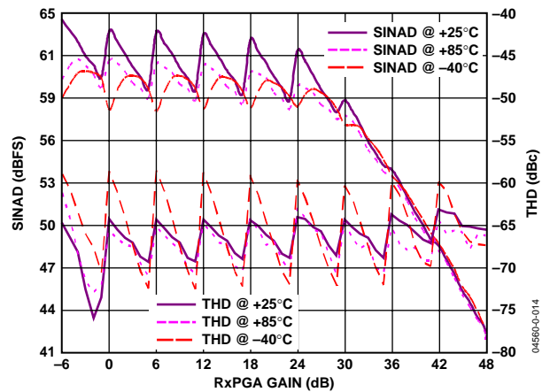
Figure 14. SINAD/THD Performance vs. RxPGA Gain and Temperature ( f_{IN} = 10\text{ MHz} )
