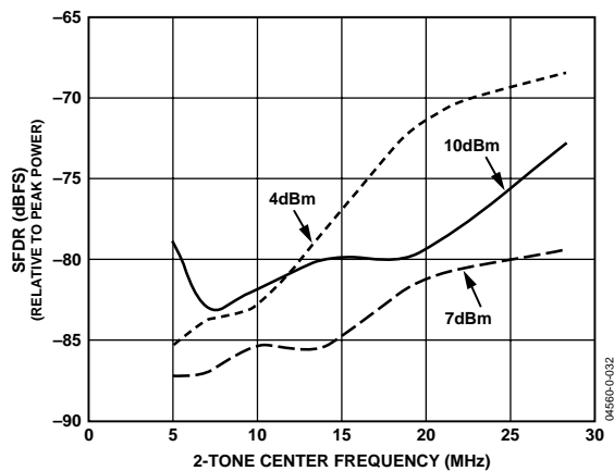
Figure 32. 2-Tone Worst Spur Frequency Sweep vs. Peak Power with f_{\text{DATA}} = 80 \text{ MSPS} , 2× Interpolation
