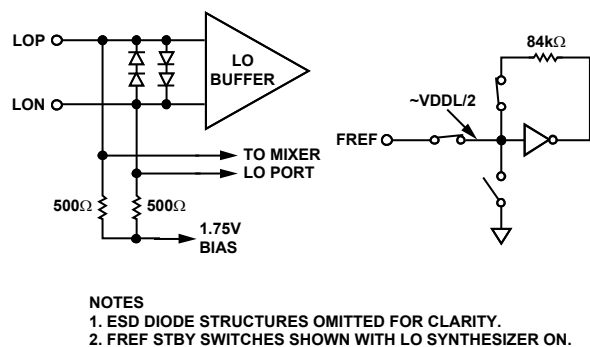
Figure 39. Equivalent Input of LO and REF Buffers
