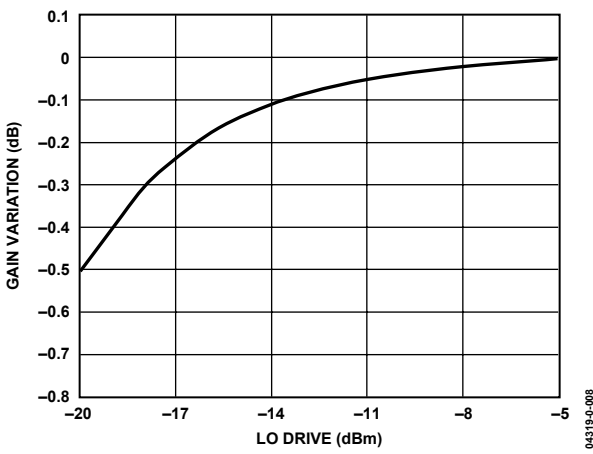
Figure 8. Normalized Gain Variation vs. LO Drive (VDDx = 3.0 V)
