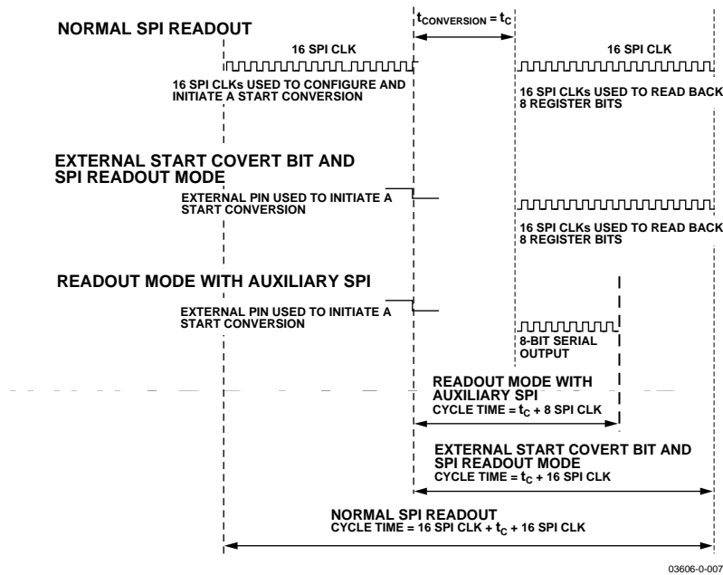
Figure 77. AuxADC Data Cycle Times for Various Readout Methods
