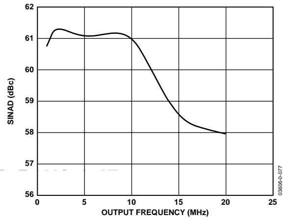
Figure 50. AD9861 Tx Path SINAD vs. Output Frequency of Tx Path, with 2 mA Full-Scale Output into 600 \Omega Differential Load
