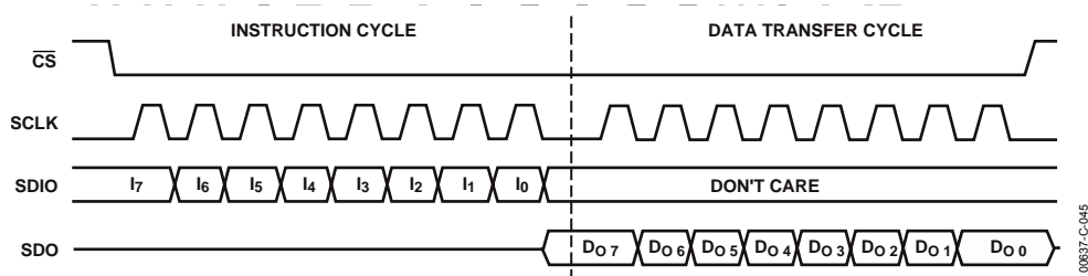
Figure 45. Three-Wire Serial Port Read Timing—Clock Stall Low
