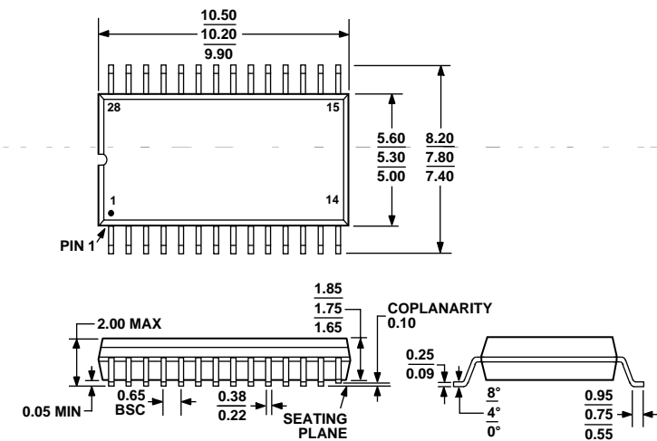
Figure 19. 28-Lead Shrink Small Outline Package [SSOP] (RS-28)
