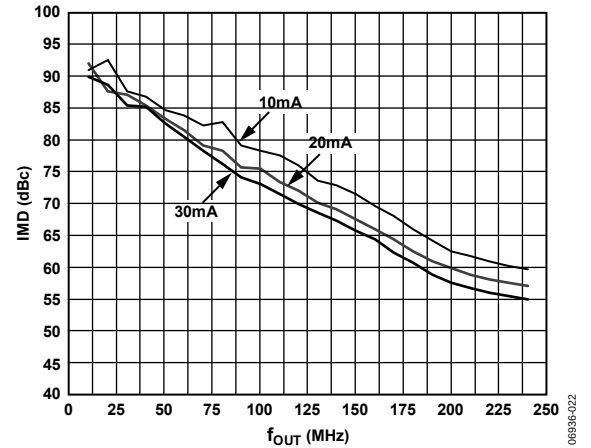
Figure 22. AD9783 IMD vs. f_{OUT} Over Analog Output, T_A = 25^\circ\text{C} , at 500 MSPS
