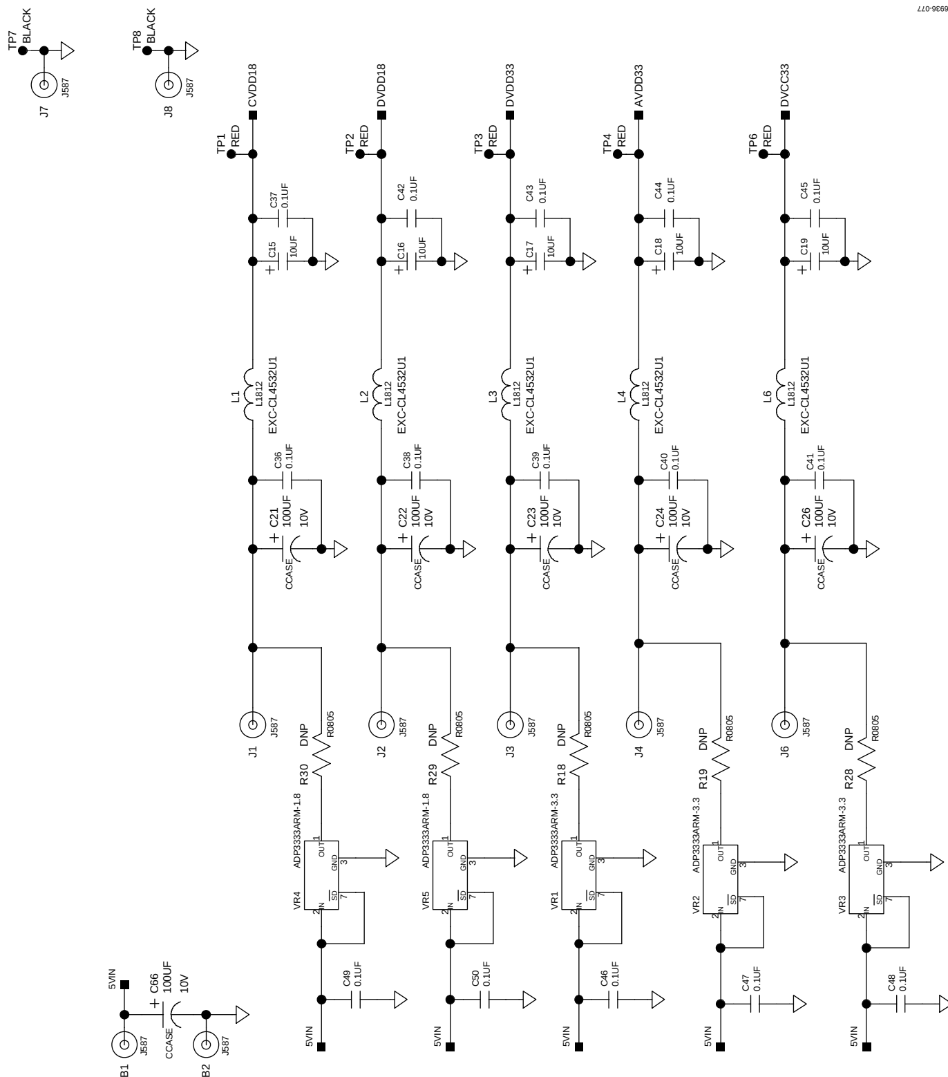
Figure 74. Power Distribution
