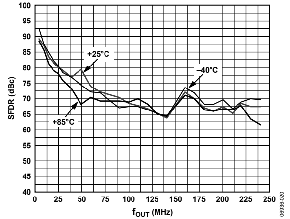
Figure 20. AD9783 SFDR vs. f_{OUT} Over Temperature, at 500 MSPS, FS = 20\text{ mA}
