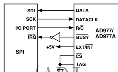
Figure 29. AD977/AD977A to SPI Interface
