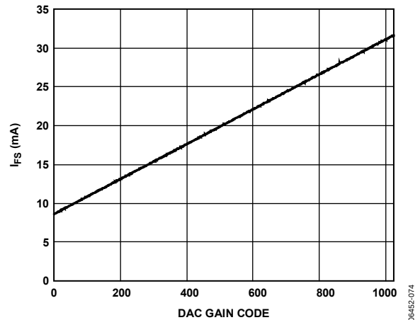
Figure 76. I_{\text{FS}} vs. DAC Gain Code
