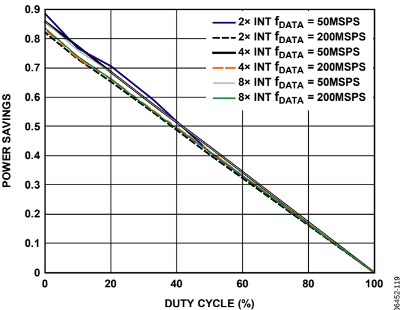
Figure 100. Power Savings Based on Duty Cycle of TXENABLE (If the TxEnable Invert bit (Register 0x02, Bit 1) is set, the function of the TXENABLE pin is inverted)
