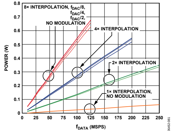
Figure 96. Power Dissipation, Digital 1.8 V Supply, I and Q Data, Dual DAC Mode, Does Not Include Zero Stuffing
