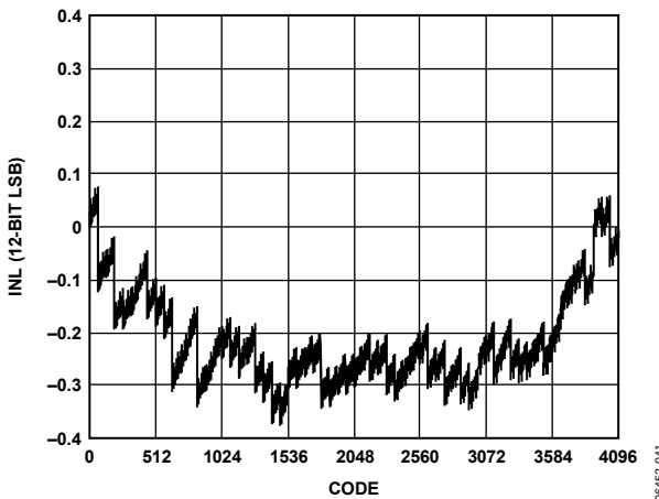
Figure 44. AD9776A Typical INL
