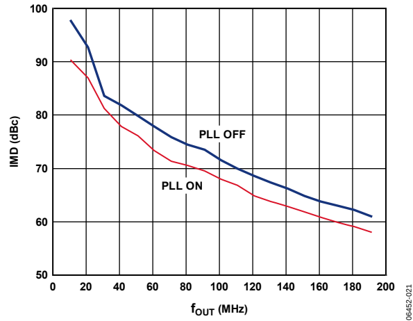
Figure 22. AD9779A Third-Order IMD vs. f_{OUT} , 4x Interpolation, f_{DATA} = 100 MSPS, PLL On vs. PLL Off
