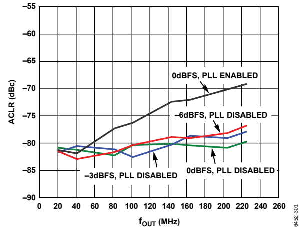
Figure 33. AD9779A ACLR for Second Adjacent Band W-CDMA, 4x Interpolation, f_{DATA} = 122.88 MSPS; On-Chip Modulation Translates Baseband Signal to IF
