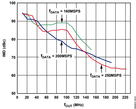
Figure 19. AD9779A Third-Order IMD vs. f_{OUT} , 2x Interpolation
