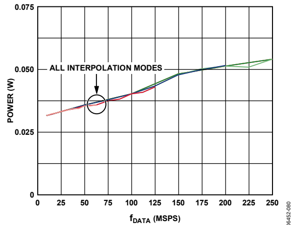
Figure 94. Power Dissipation, Digital 3.3 V Supply, I Data Only, Real Mode, Includes Modulation Modes and Zero Stuffing
