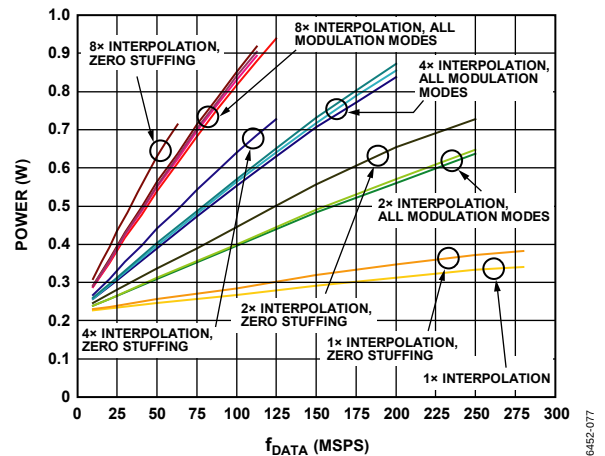
Figure 95. Total Power Dissipation, Dual DAC Mode
