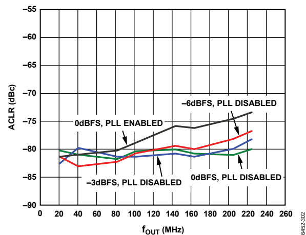
Figure 34. AD9779A ACLR for Third Adjacent Band W-CDMA, 4x Interpolation, f_{DATA} = 122.88 MSPS, On-Chip Modulation Translates Baseband Signal to IF
