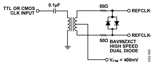
Figure 73. TTL or CMOS REFCLK Drive Circuit
