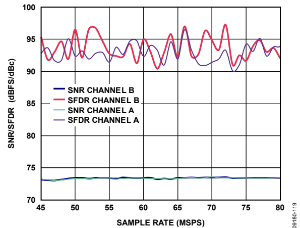
Figure 19. AD9644-80 Single-Tone SNR/SFDR vs. Sample Rate ( f_s ) with f_{IN} = 70. MHz
